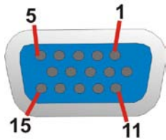
Figure 3-21: VGA Connector
