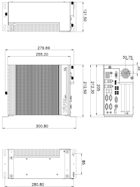
Figure 1-10: TANK-870-Q170-2 slot Physical Dimensions (millimeters)
