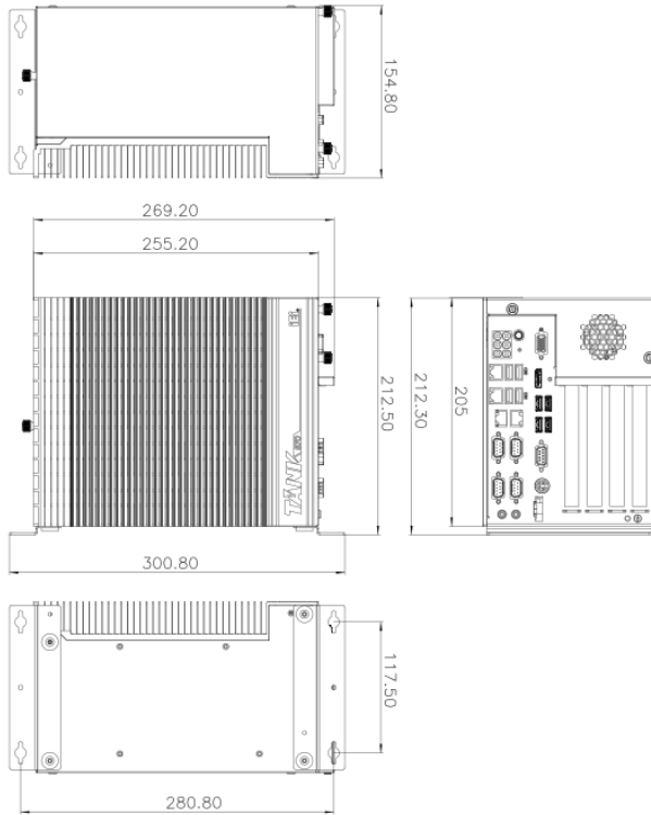
Figure 1-11: TANK-870-Q170-4 slot Physical Dimensions (millimeters)
