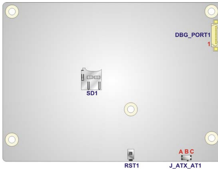
Figure 4-2: System Motherboard (Rear)
