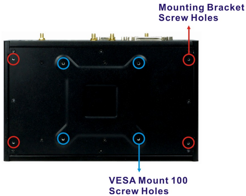
Figure 1-5: Bottom Panel
