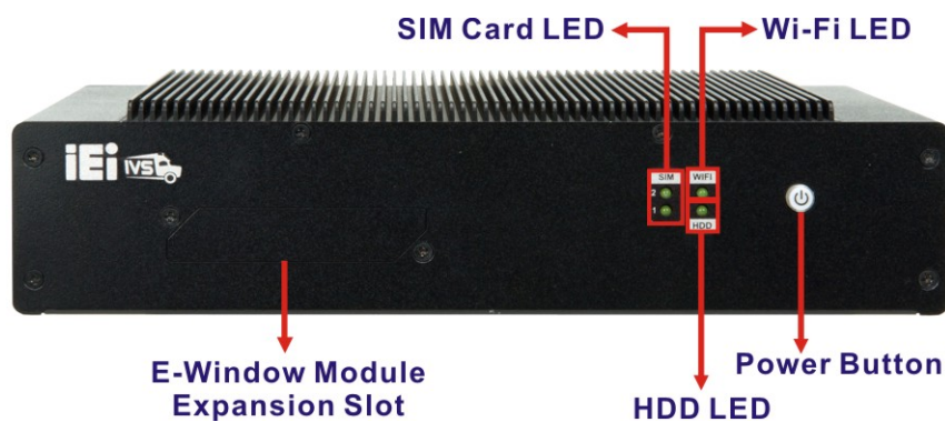
Figure 1-2: Front Panel
