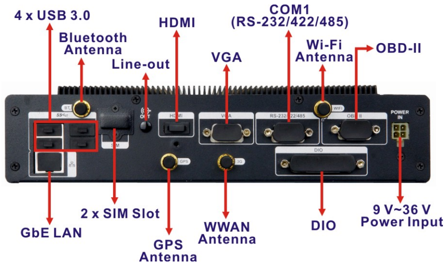
Figure 1-4: Rear Panel
