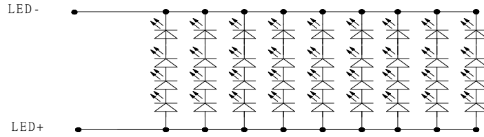
CIRCUIT DIAGRAM (4串9并)
