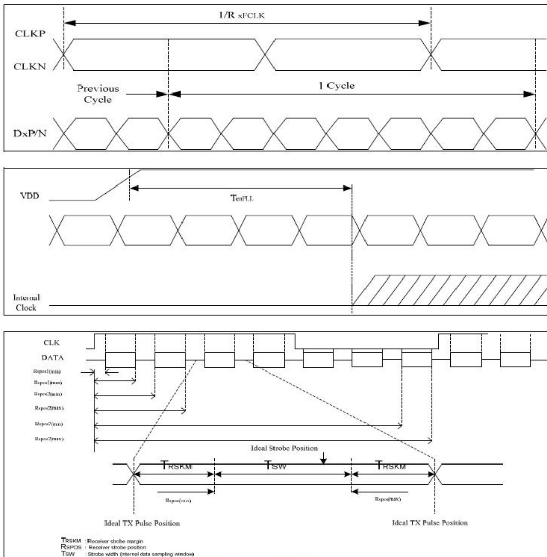
Figure 13.3: LVDS figure
