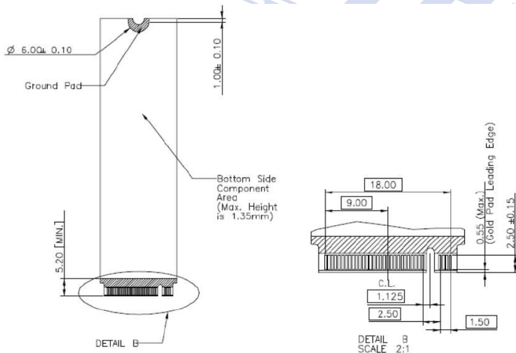
Bottom View
